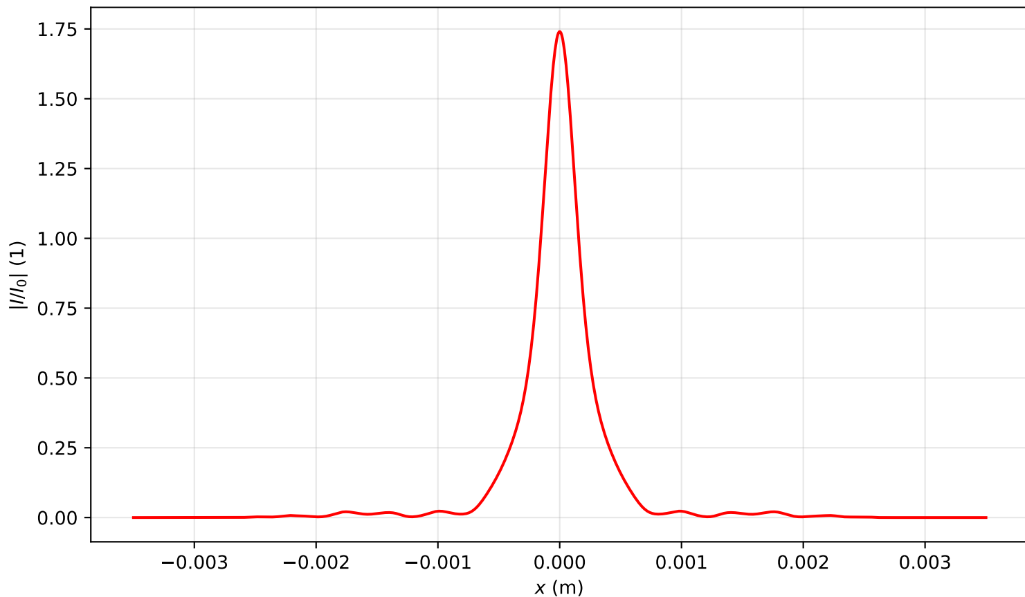
Intensity profile I(x, y = 0, z = 2.388)/I_0 , P_{in}=3.0P_{cr} , artificial time
